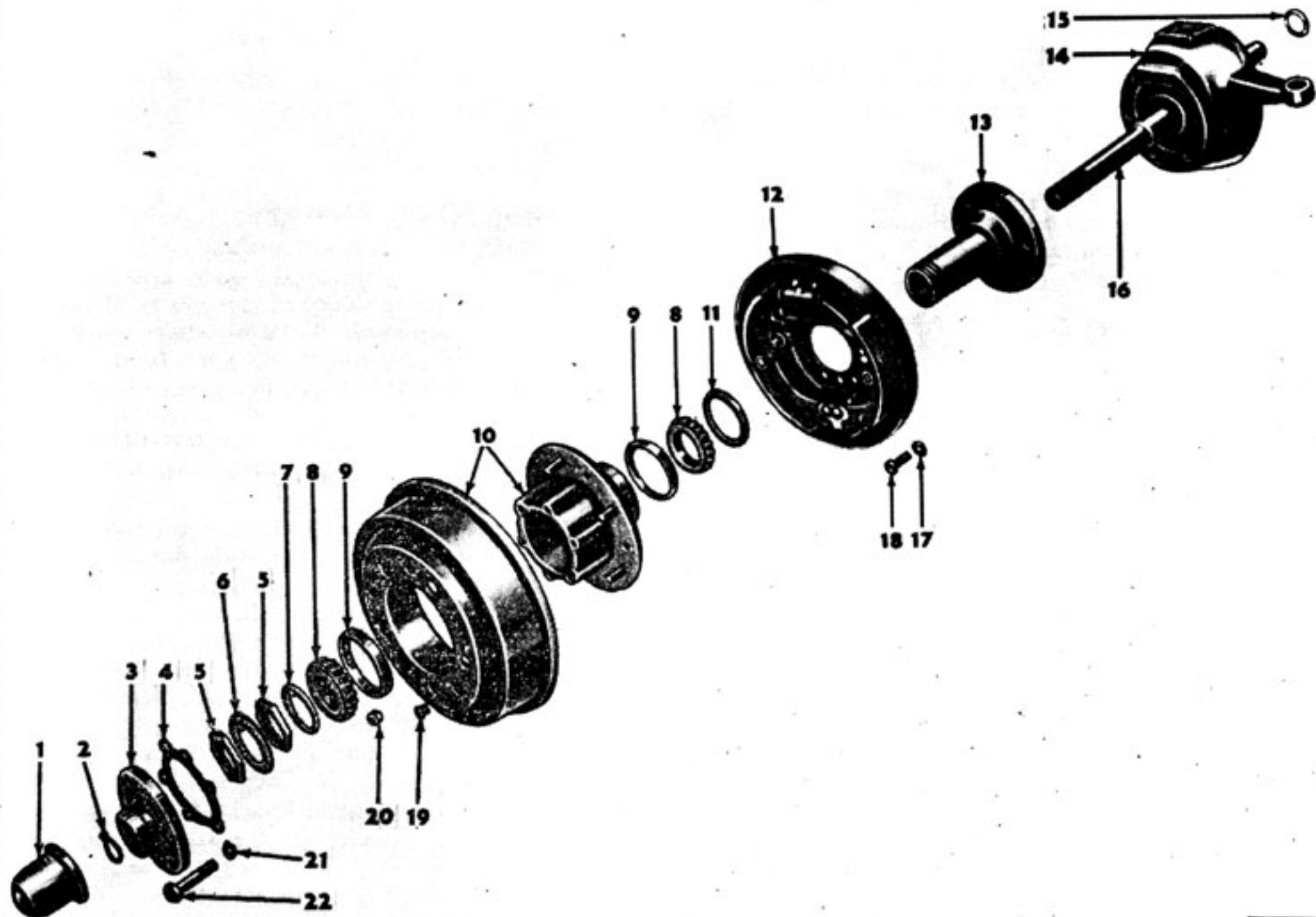
FIG. 292—FRONT WHEEL AND ATTACHING PARTS
