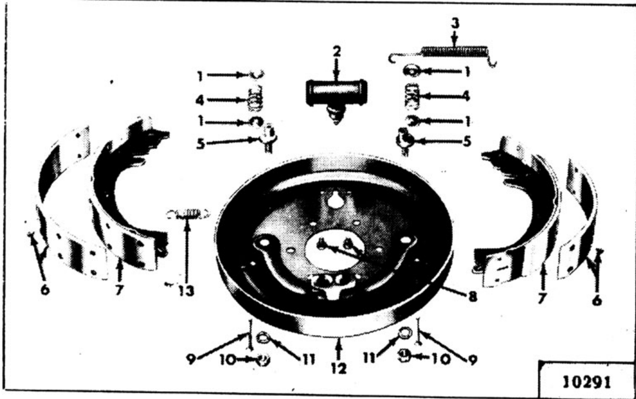
FIG. 288—WHEEL BRAKE
